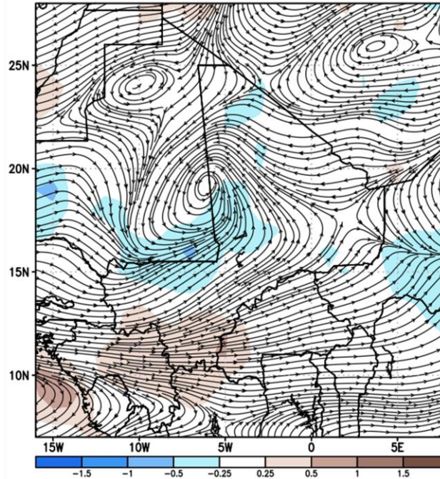
GEFS Week-1 700-hPa Divergence and Wind Anomaly Valid: 20250724 - 20250730
