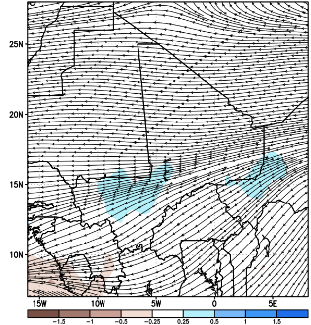
GEFS Week-2 200-hPa Divergence and Wind Anomaly Valid: 20250731 - 20250806
