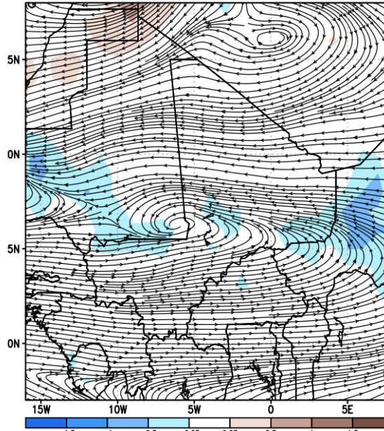
GEFS Week-2 700-hPa Divergence and Wind Anomaly Valid: 20250731 - 20250806
