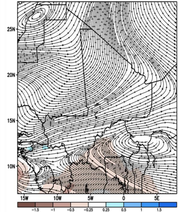
GEFS Week-1 200-hPa Divergence and Wind Anomaly Valid: 20250724 - 20250730
