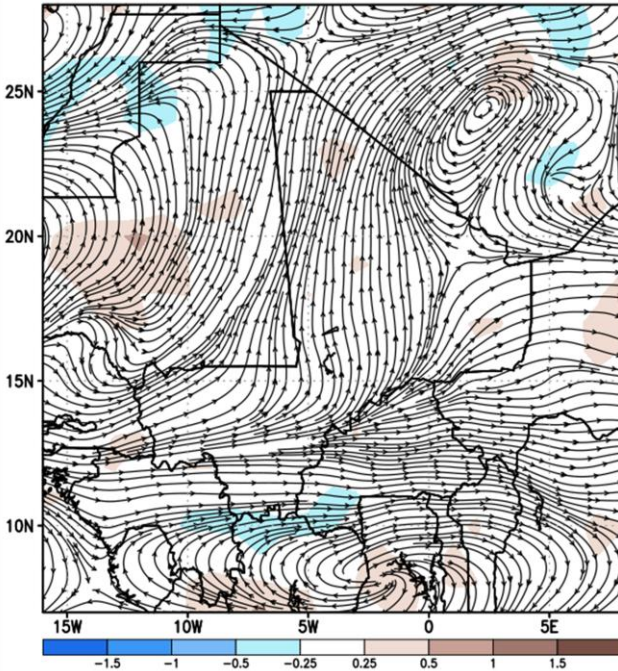
GEFS Week-1 850-hPa Divergence and Wind Anomaly Valid: 20250724 - 20250730
