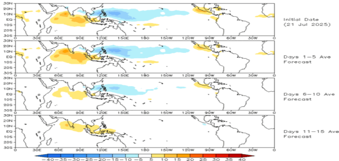
Prediction of MJO-related anomalies using GEFS operational forecast Initial date: 21 Jul 2025 OLR
