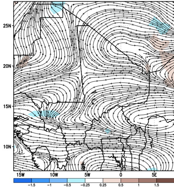
GEFS Week-2 850-hPa Divergence and Wind Anomaly Valid: 20250731 - 20250806
